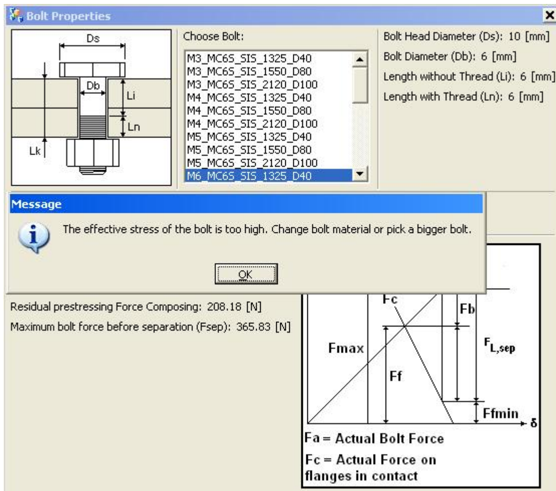
Figure 8. In this picture the result from equation 1 is found in lower left interface parameter. The figure also shows a warning message due to too high effective stress.
