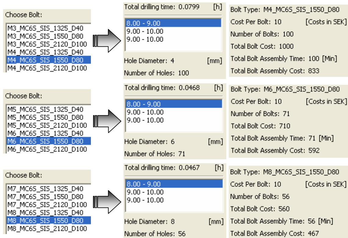
Figure 7. Choice of bolt affects the size of the hole and the number of holes which in turn affect the drilling and assemble time.
